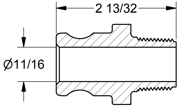
SECTION C-C SCALE 1 : 1
