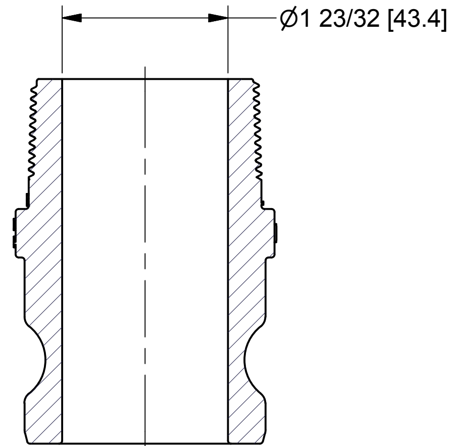
SECTION B-B SCALE 1 : 1
