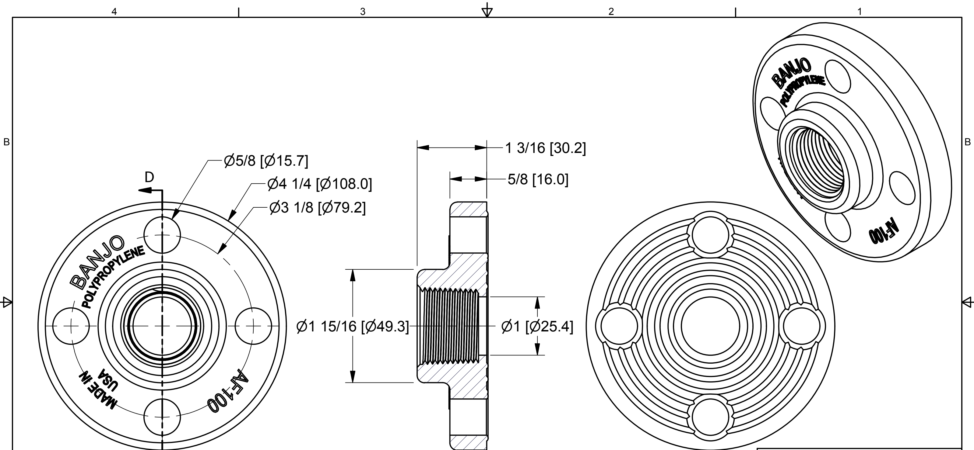
SECTION D-D SCALE 1
