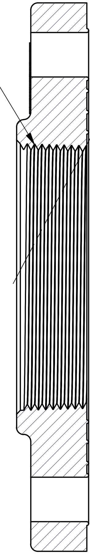
SECTION C-C SCALE 1 : 1
