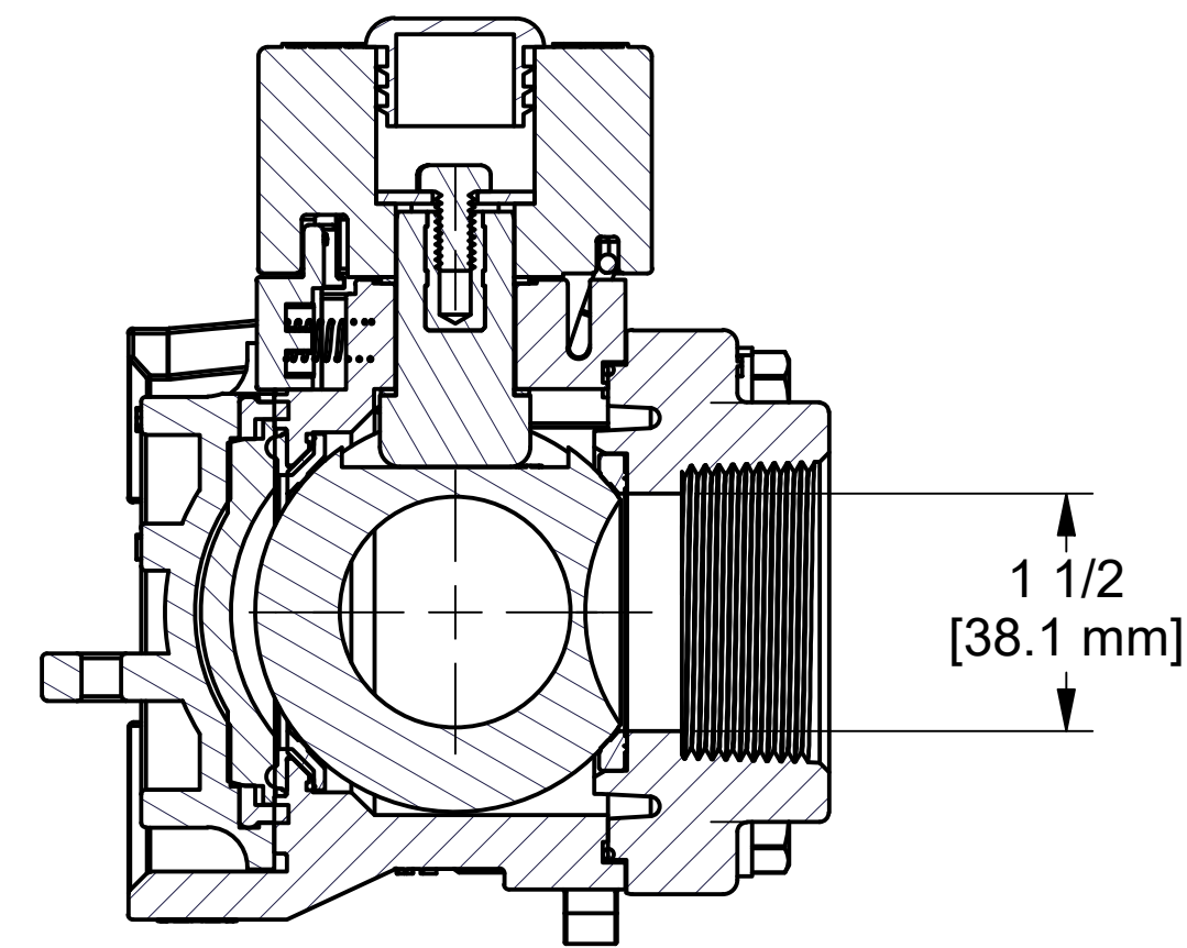
SECTION B-B SCALE 3/4
