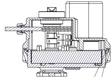
SECTION A-A SCALE 1 : 1 O-RING SEAL O-RING SEAL
