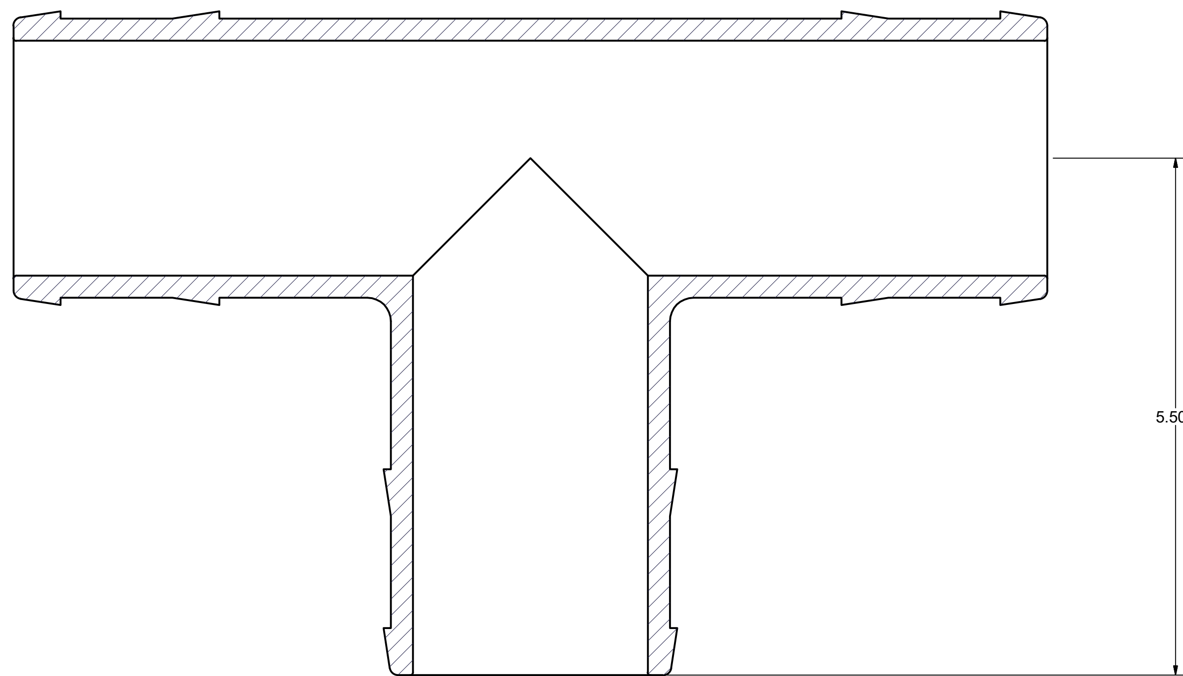
SECTION B-B SCALE 1 : 1
