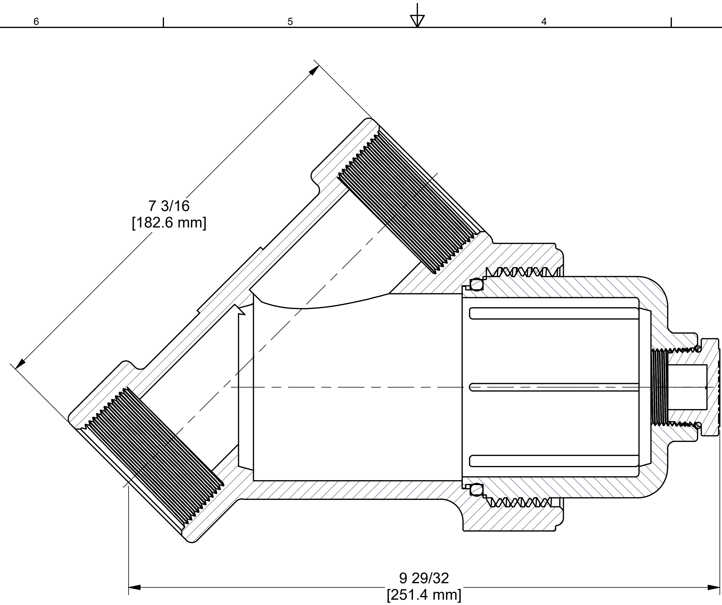
SECTION B-B SCALE 1 : 1
