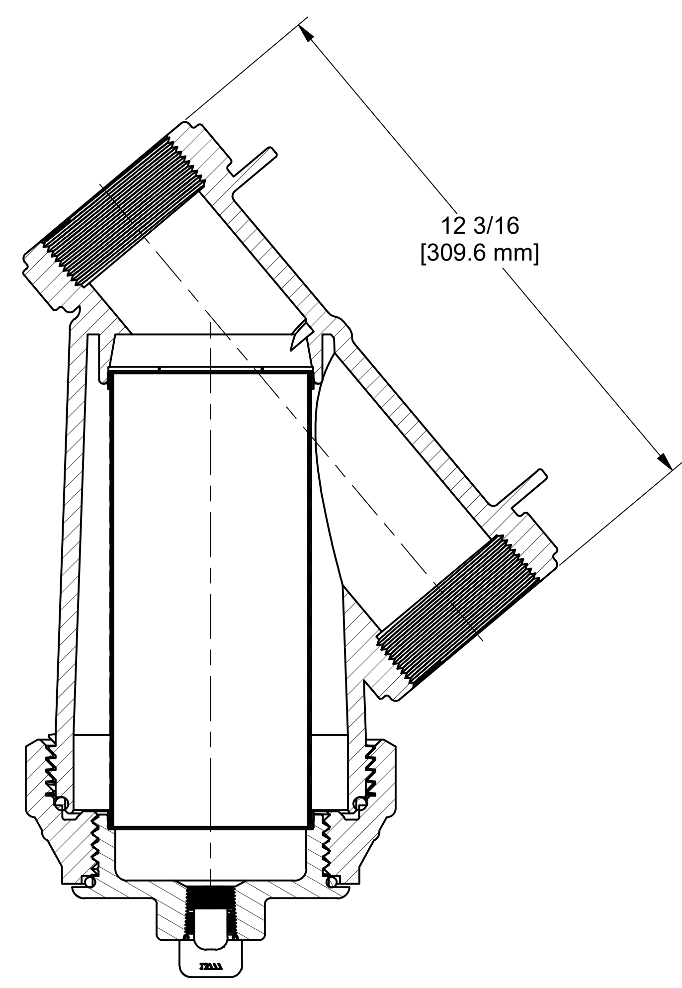
SECTION B-B SCALE 1:2
