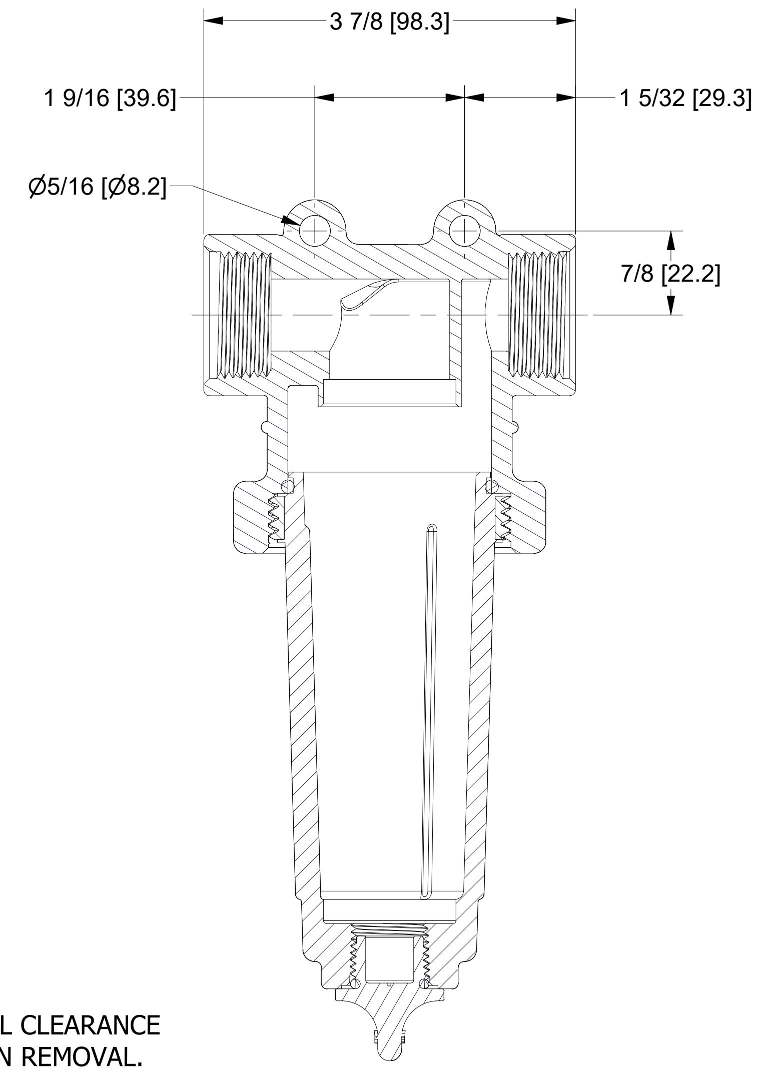
SECTION B-B SCALE 1 : 1
