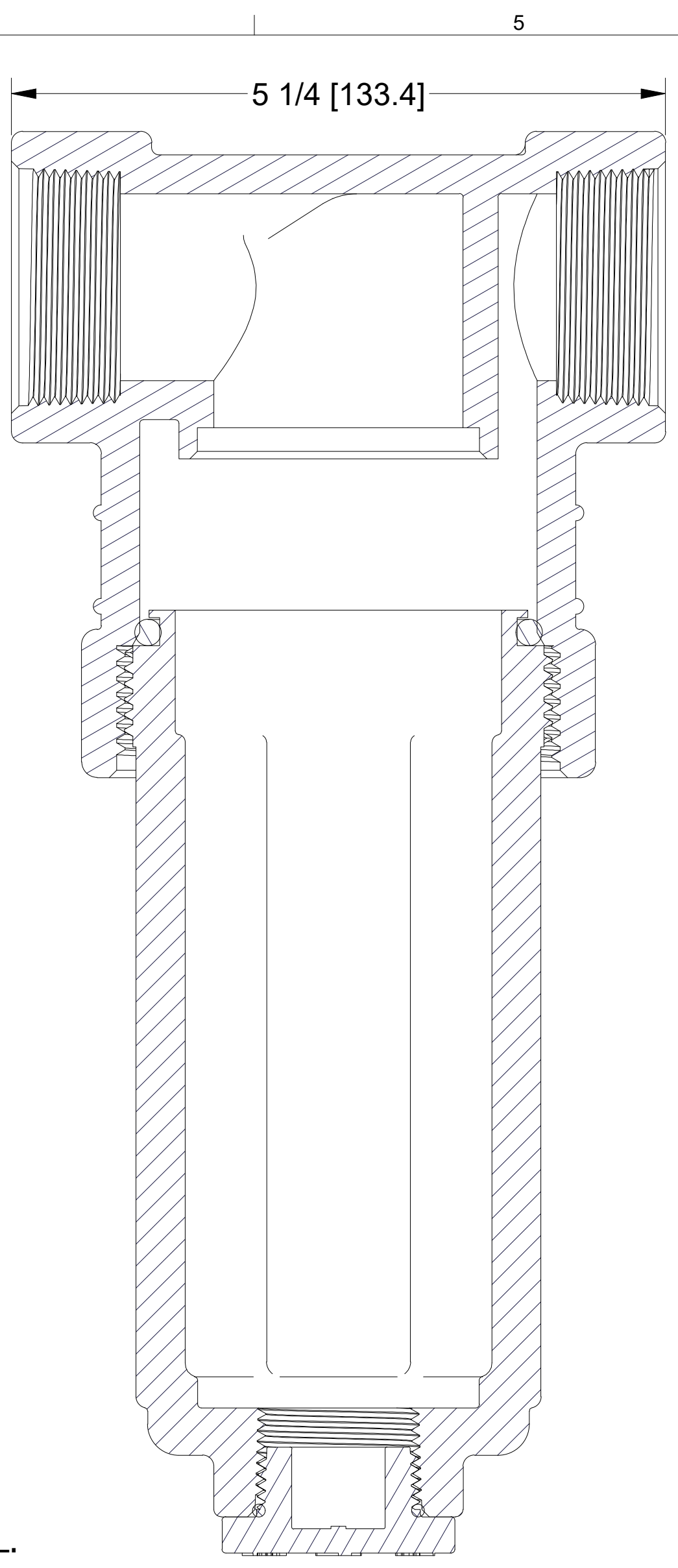
SECTION B-B SCALE 1 : 1
