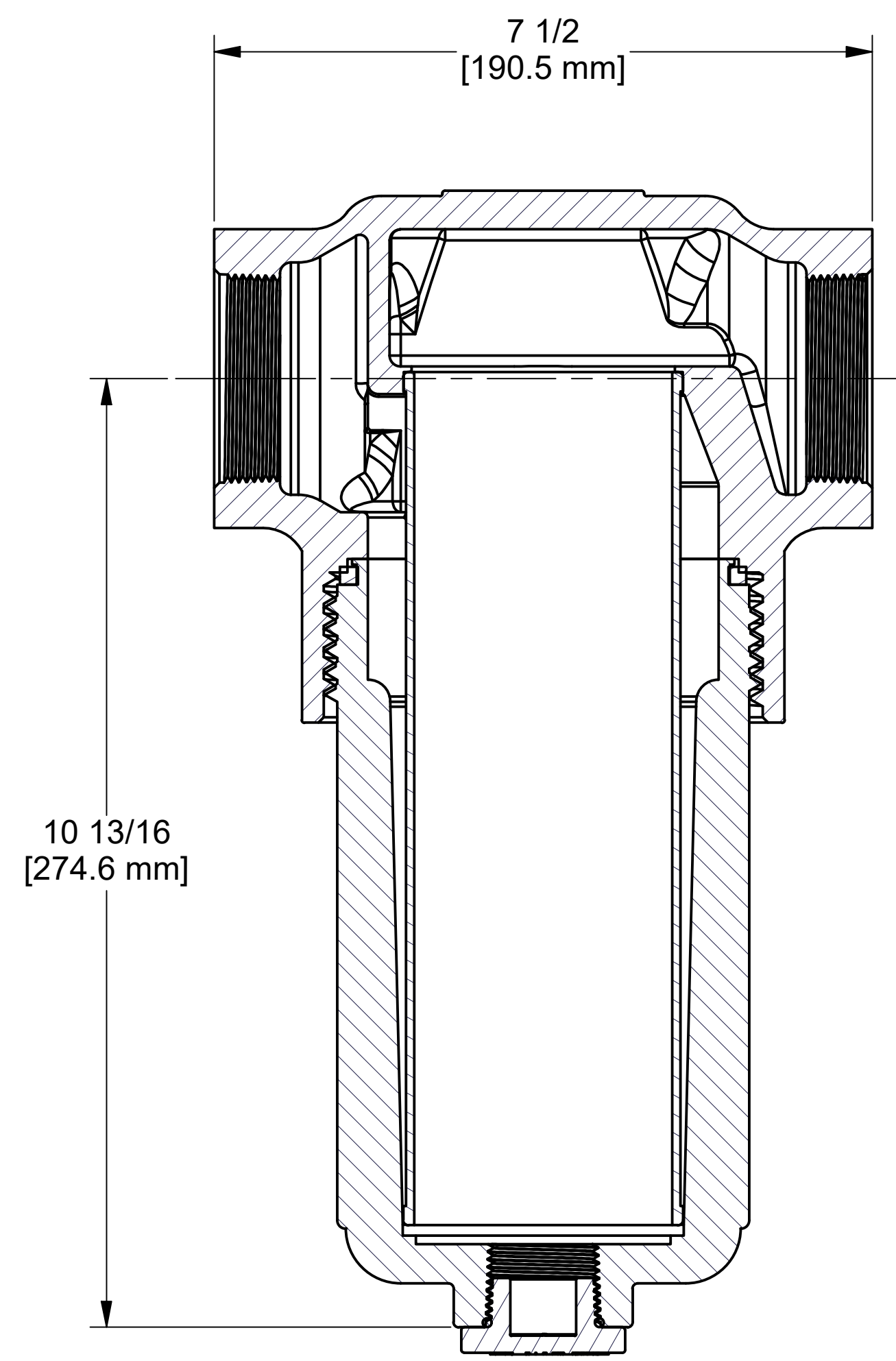
SECTION B-B SCALE 2 / 3
