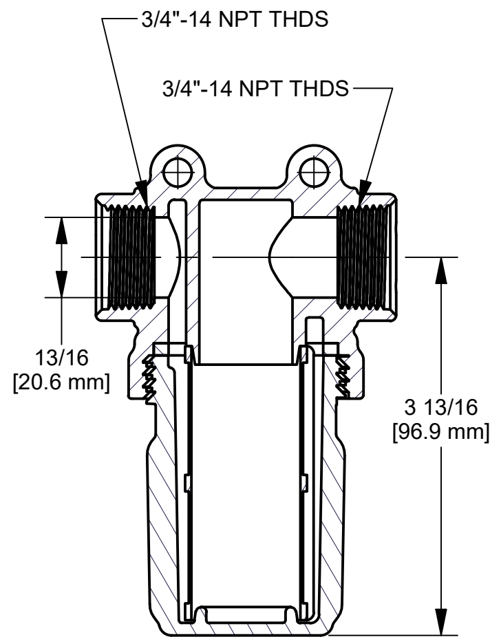
SECTION A-A SCALE 3/4
