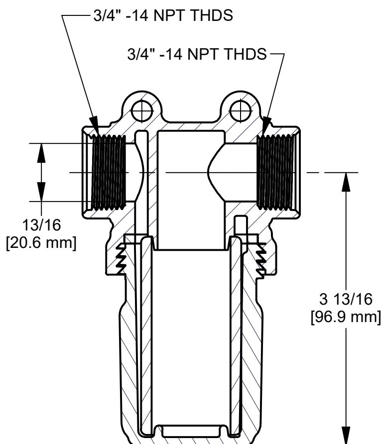
SECTION A-A SCALE 3/4
