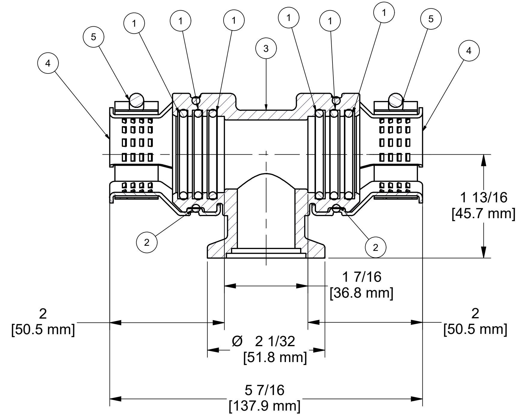
SECTION C-C SCALE 1 : 1
