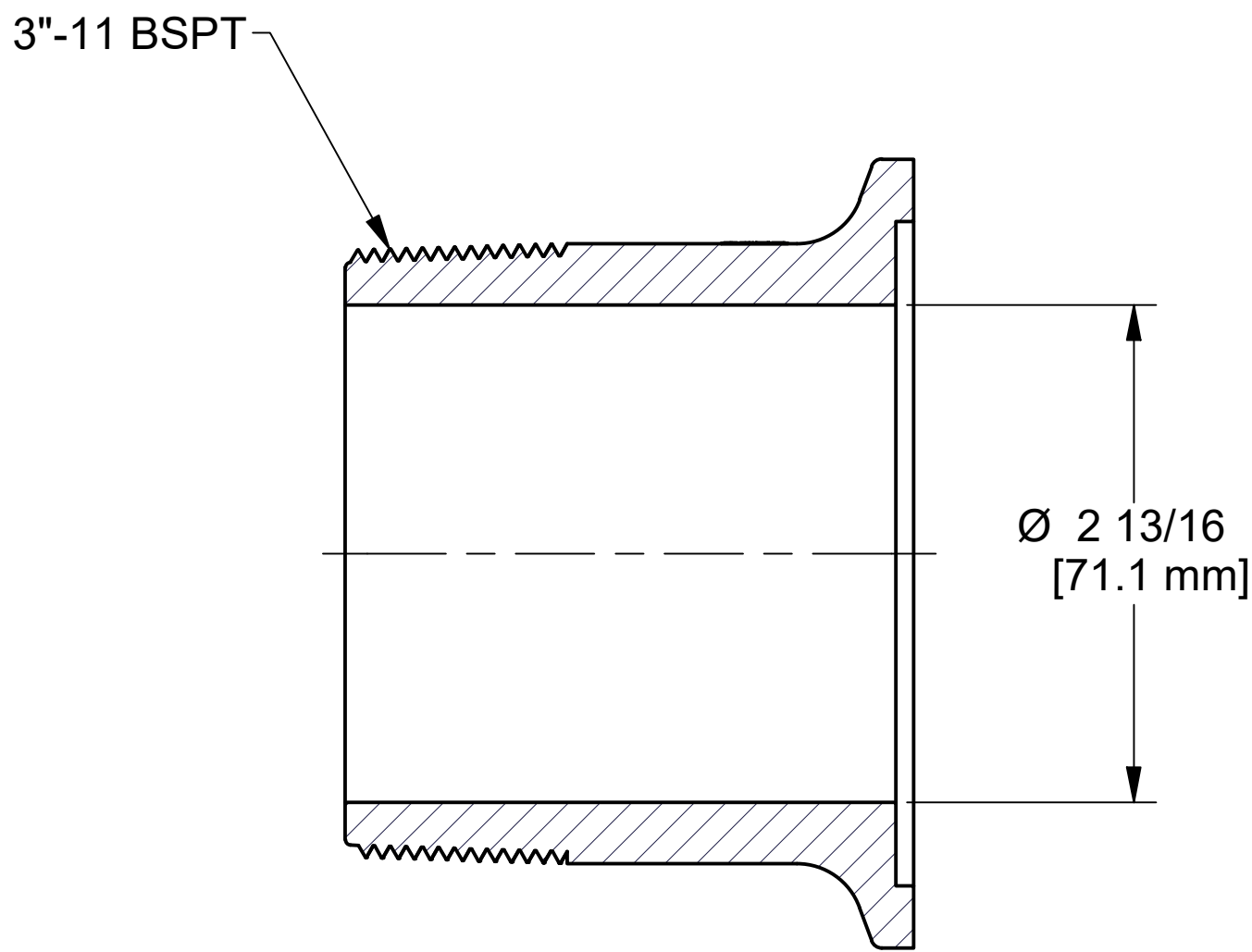
SECTION C-C SCALE 1 : 1
