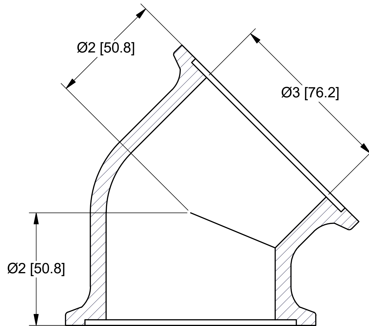
SECTION C-C SCALE 1:1
