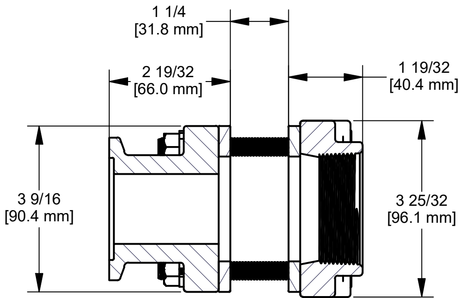
SECTION A-A SCALE 1 / 2
