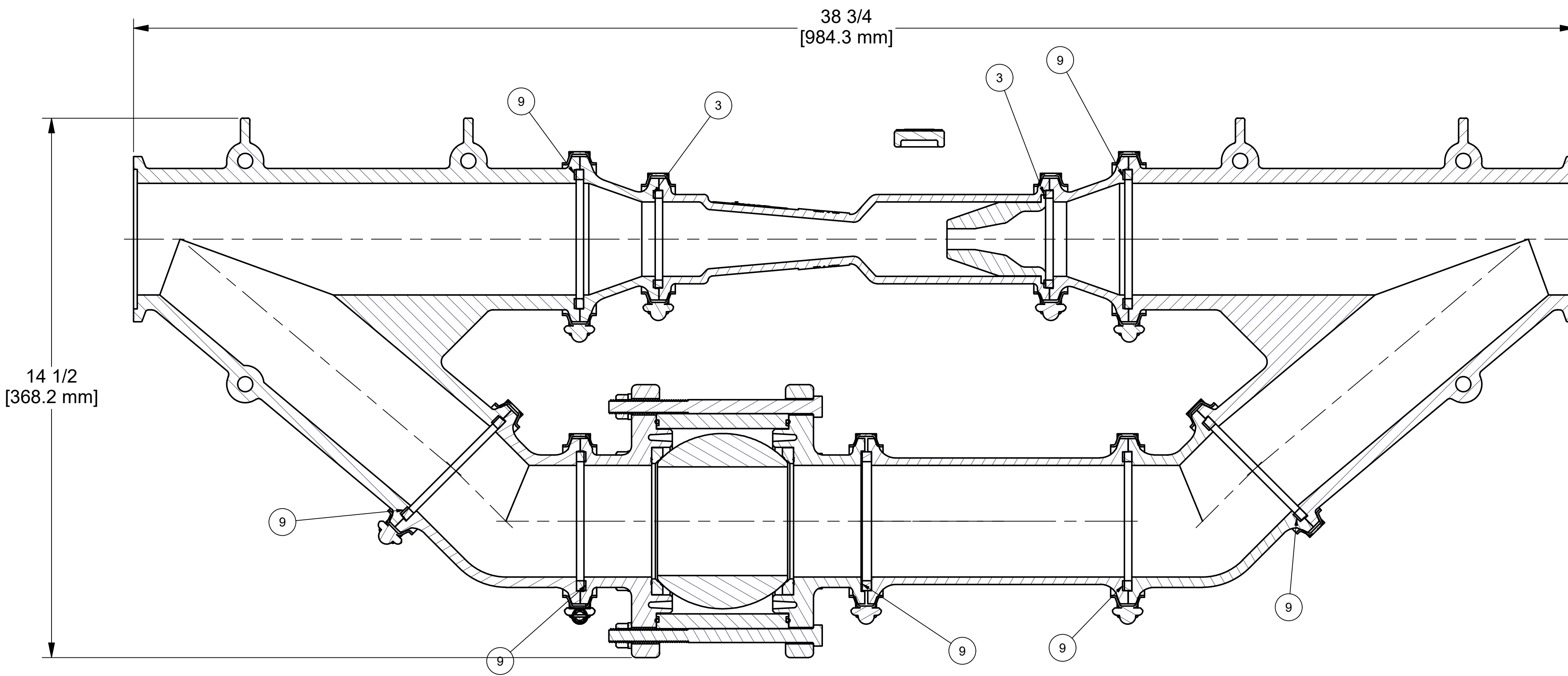
SECTION B-B SCALE 1:2
