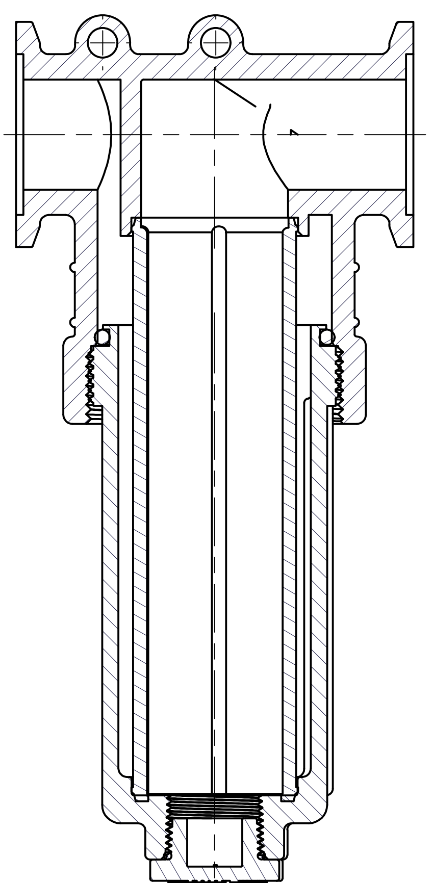
SECTION B-B SCALE 3 / 4
