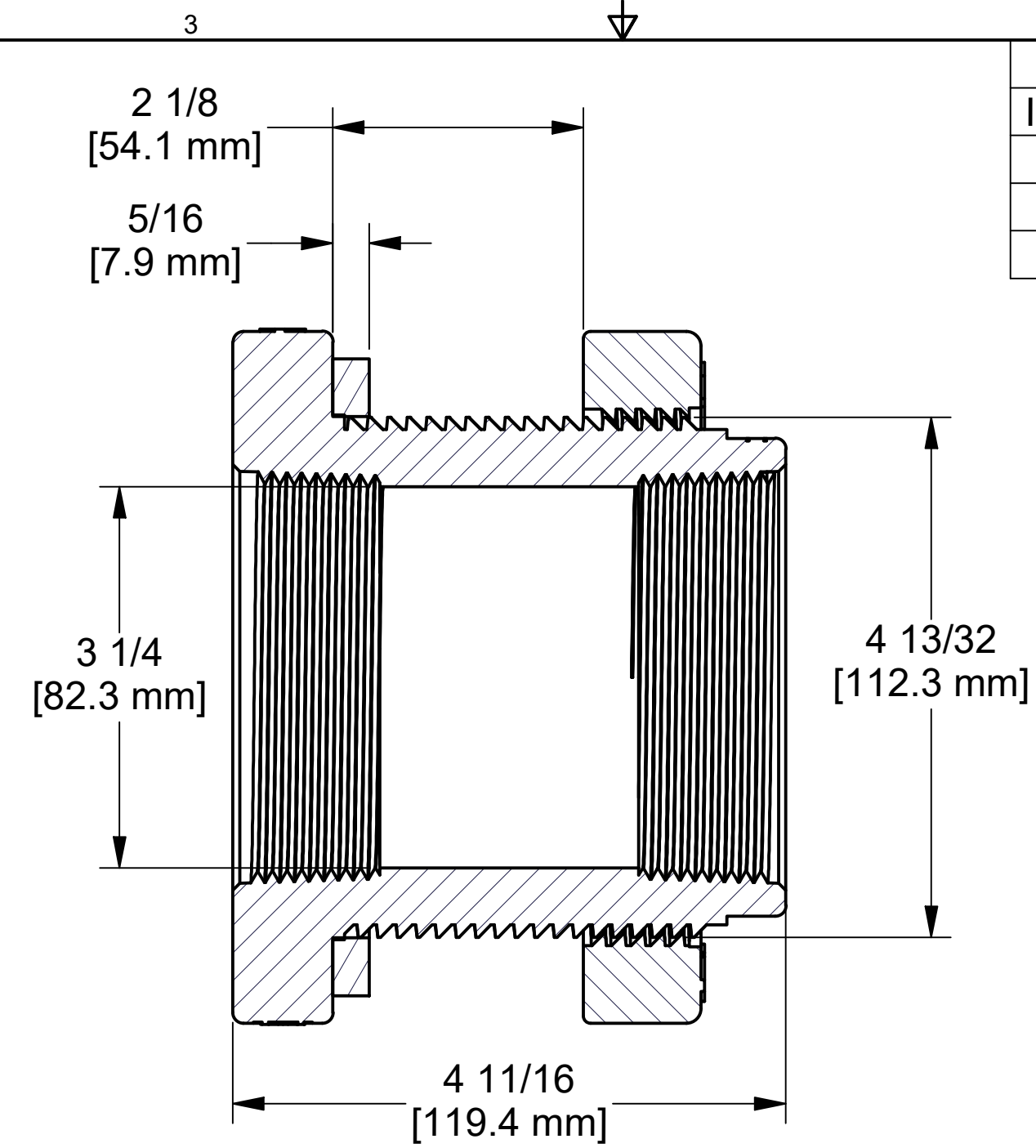
SECTION B-B SCALE .75
