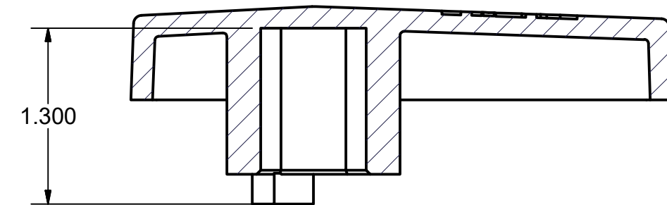
SECTION B-B SCALE 1
