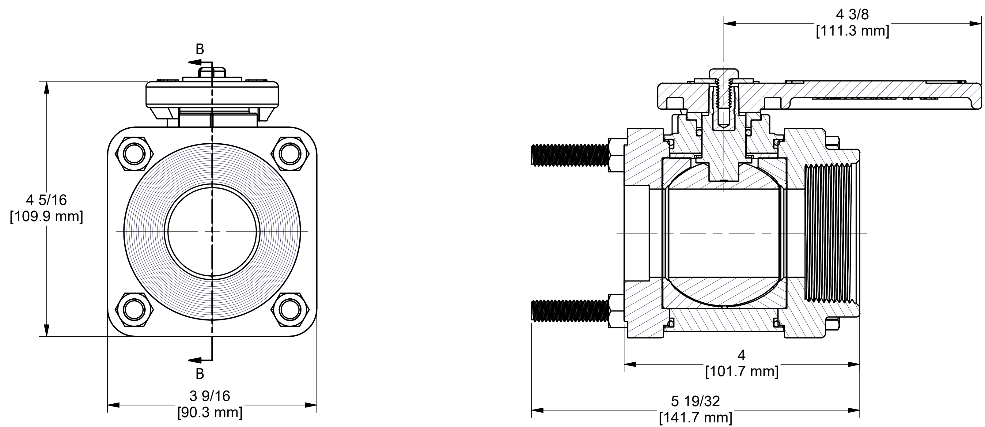
SECTION B-B SCALE 1 : 1
