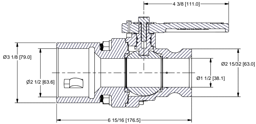
SECTION C-C SCALE 1:1
