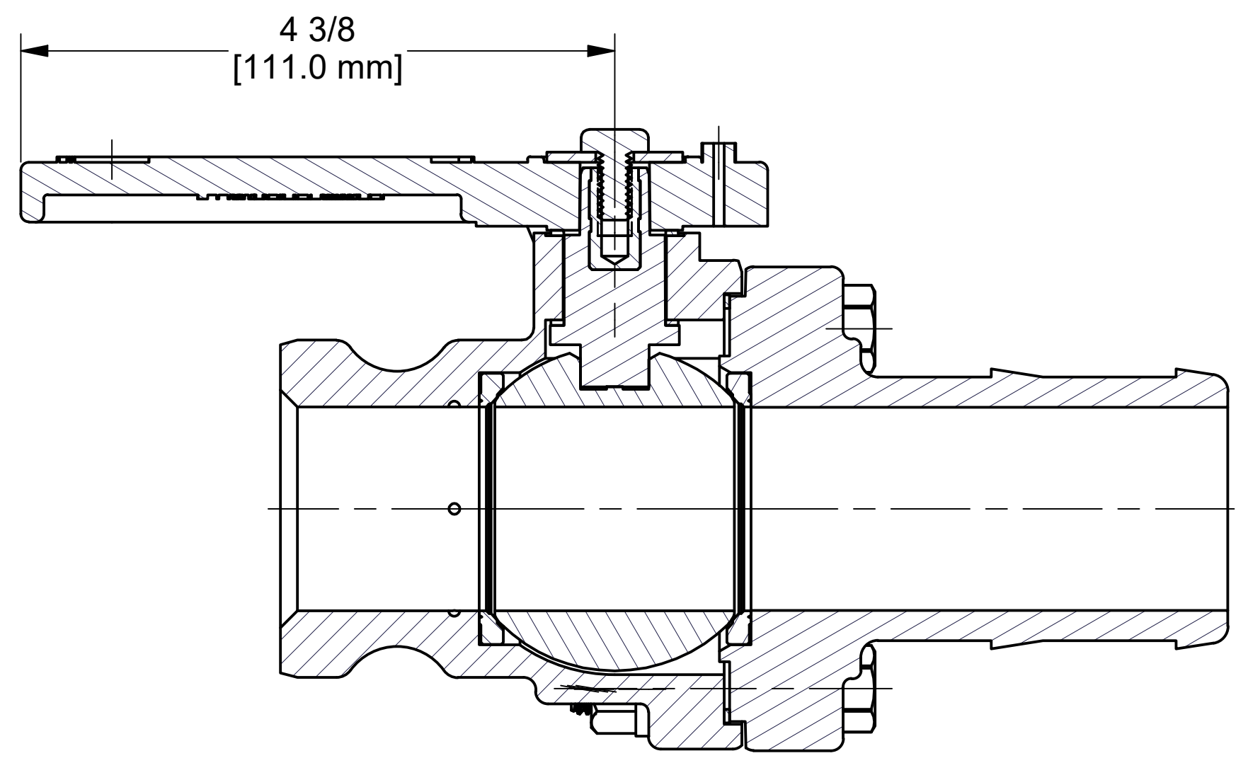
SECTION B-B
